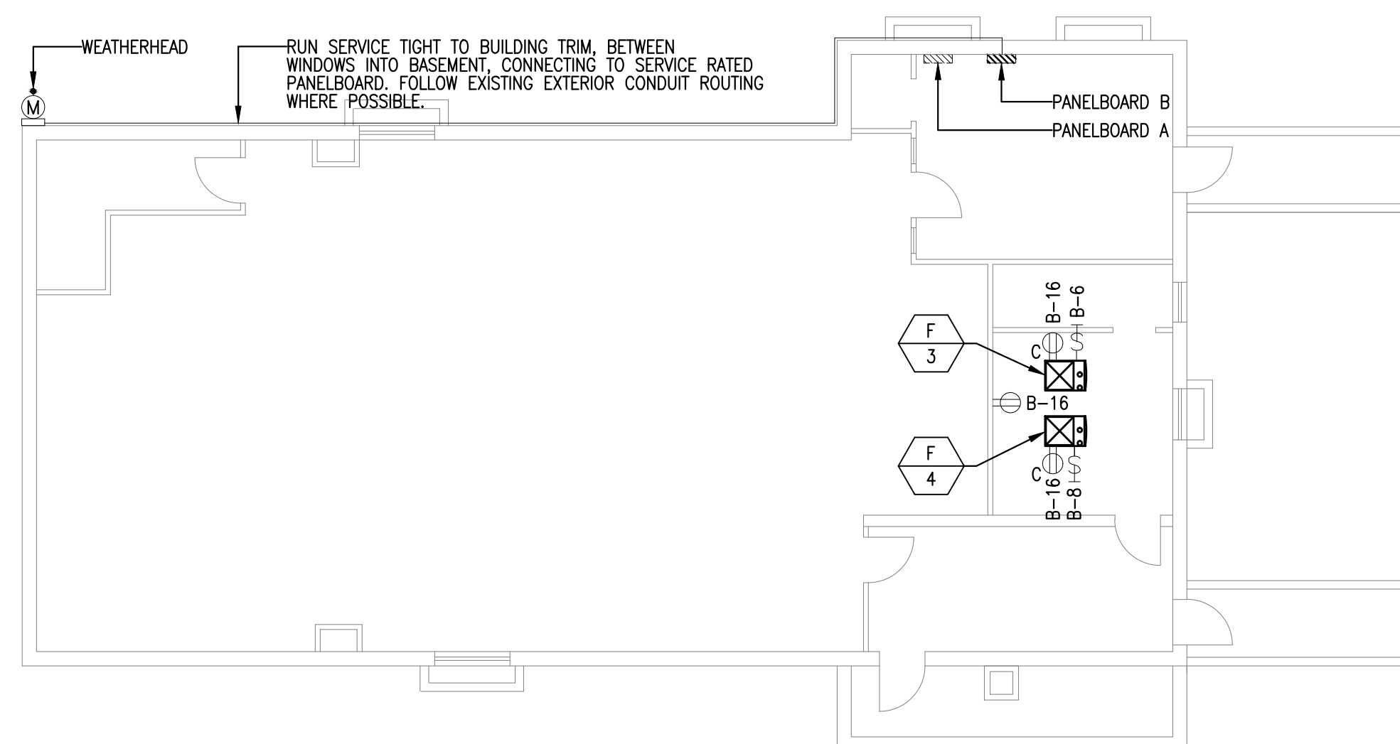
ELECTRICAL - BASEMENT PLAN
