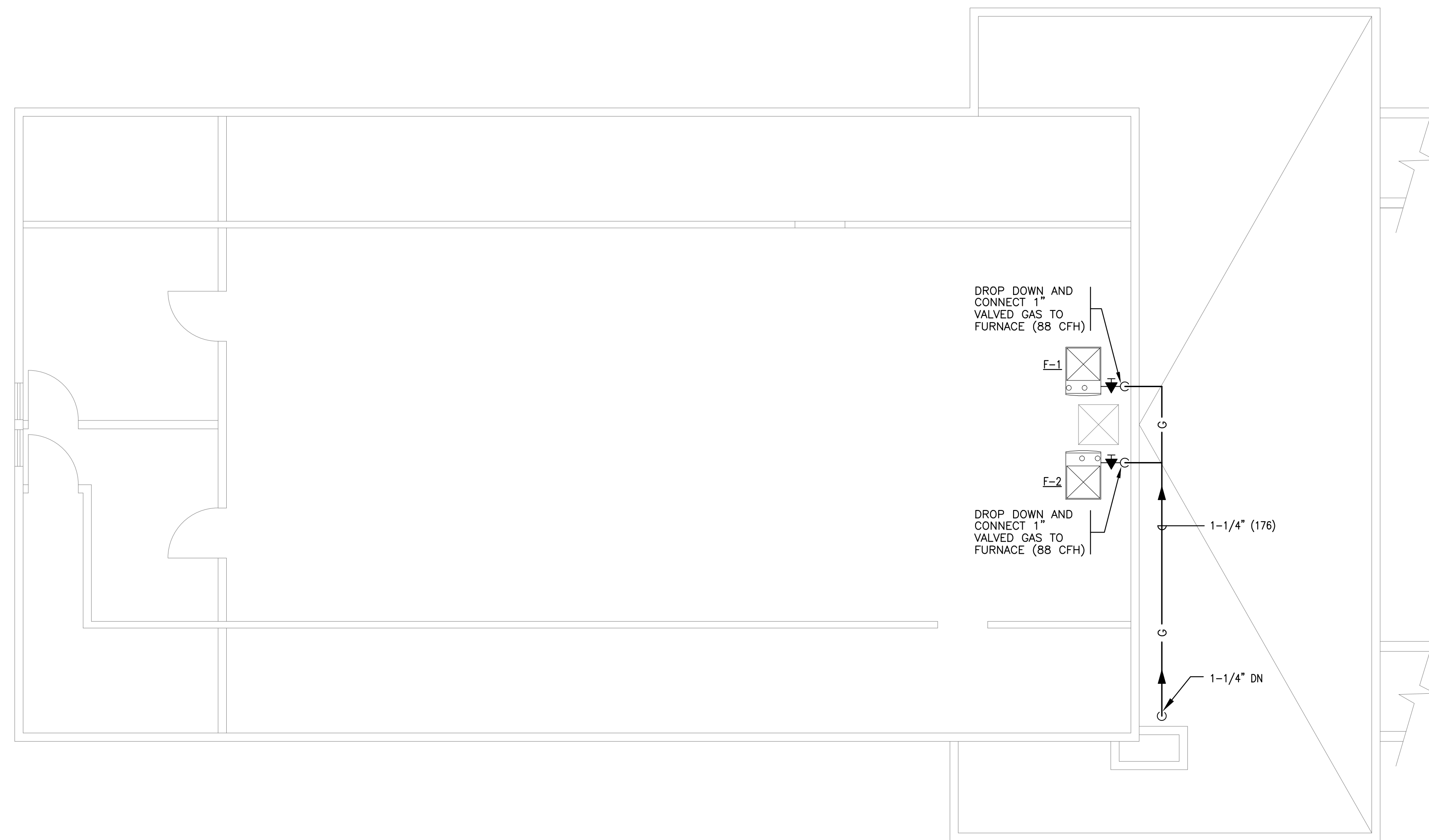
MECHANICAL - MEZZANINE GAS PIPING PLAN
