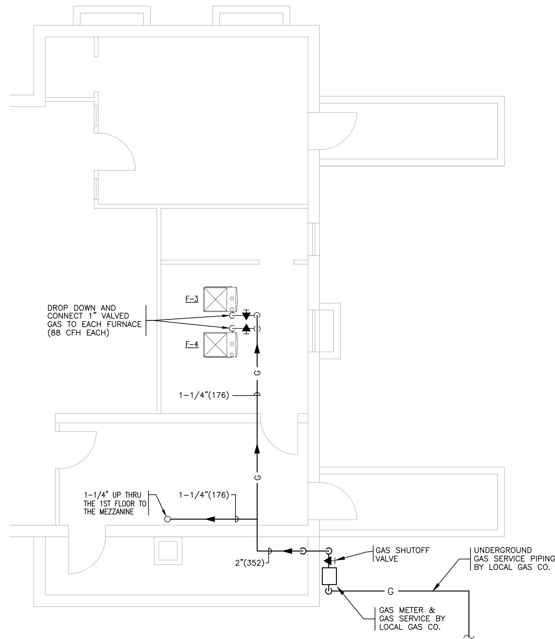
MECHANICAL - PARTIAL BASEMENT PLAN GAS PIPING
